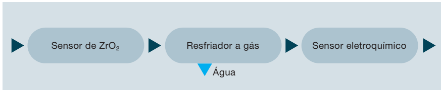
Figure 26 Configuration for measuring moisture in the flue gas
