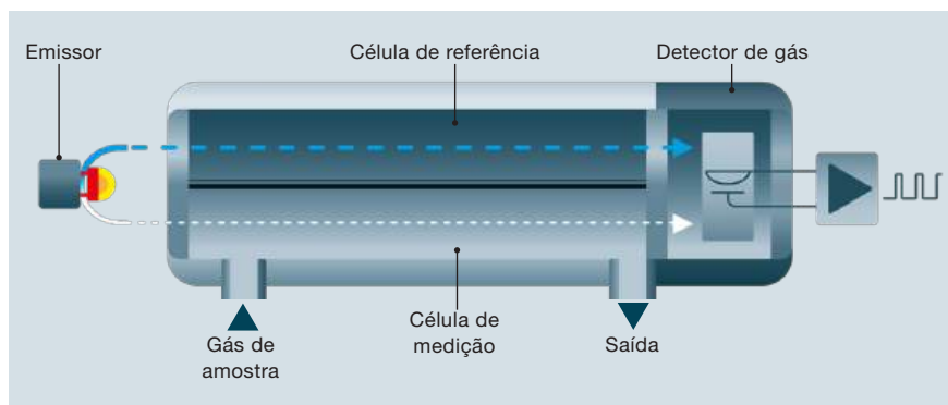
Figura 18 Sensor NDIR (design compacto)
